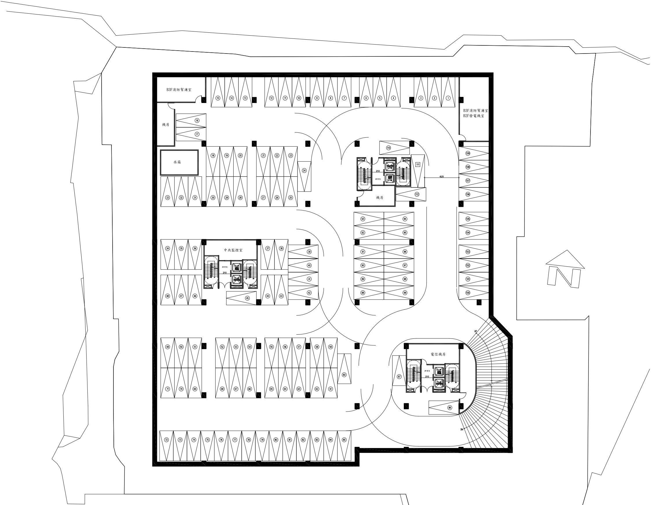
B2F-B3F PLAN S:1/400
