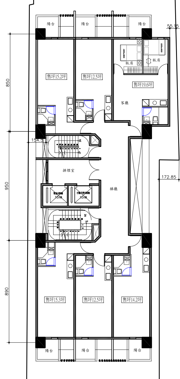
2F-20F PLAN S:1/200
