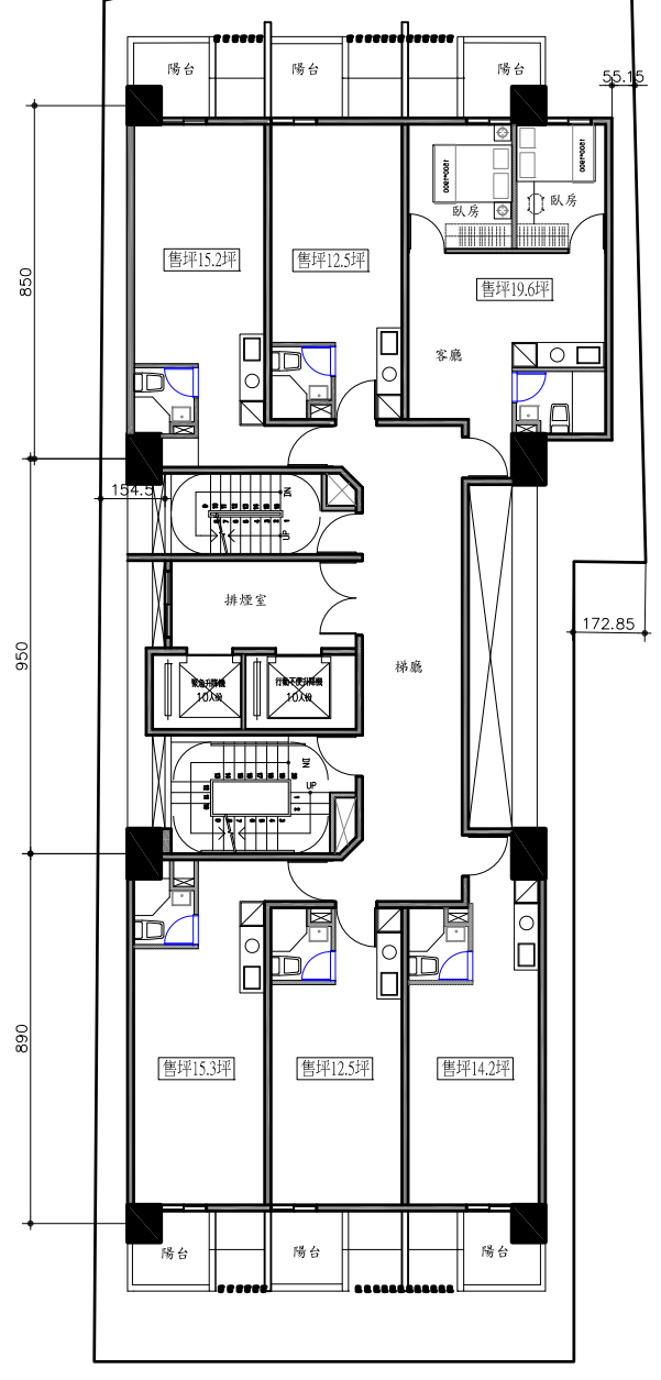
2F-20F PLAN S:1/200
