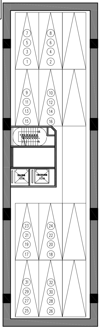
B2F-B4F PLAN S:1/200
