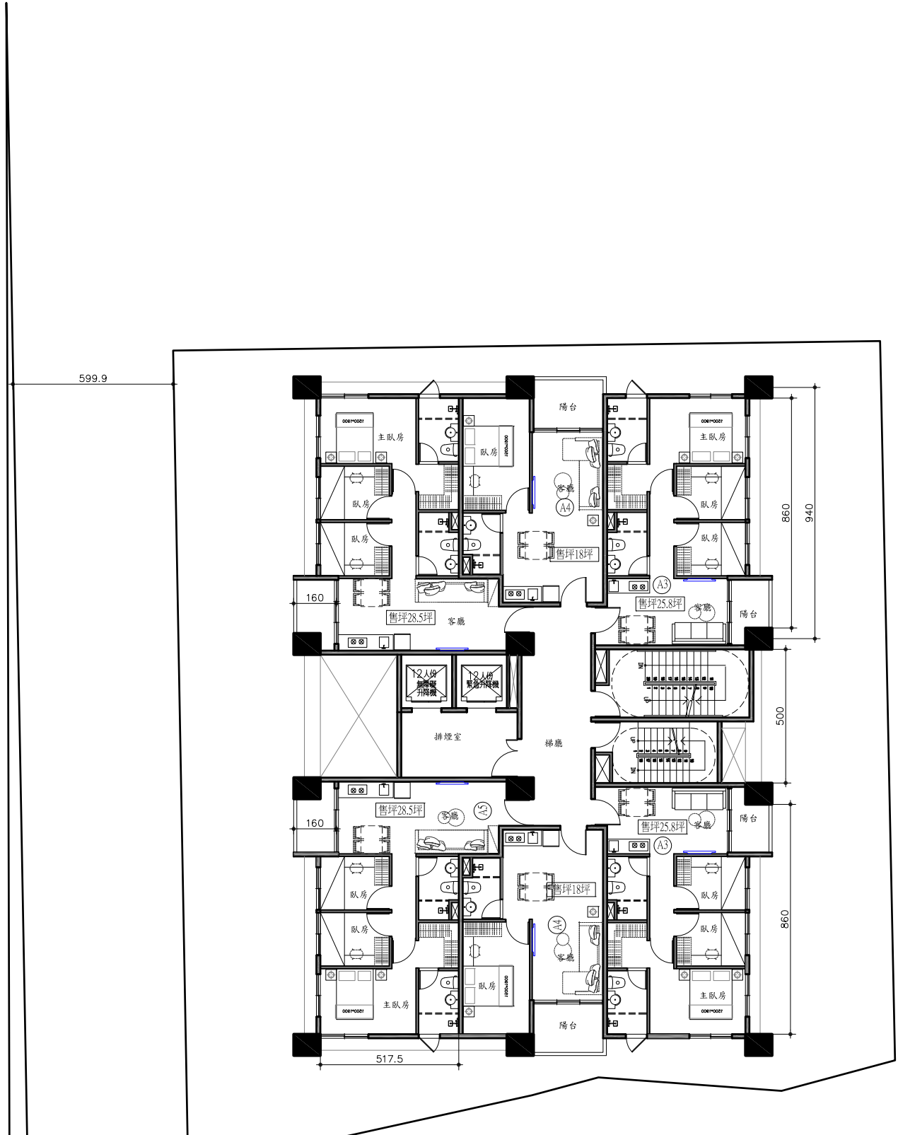
2F-12F PLAN S:1/200
